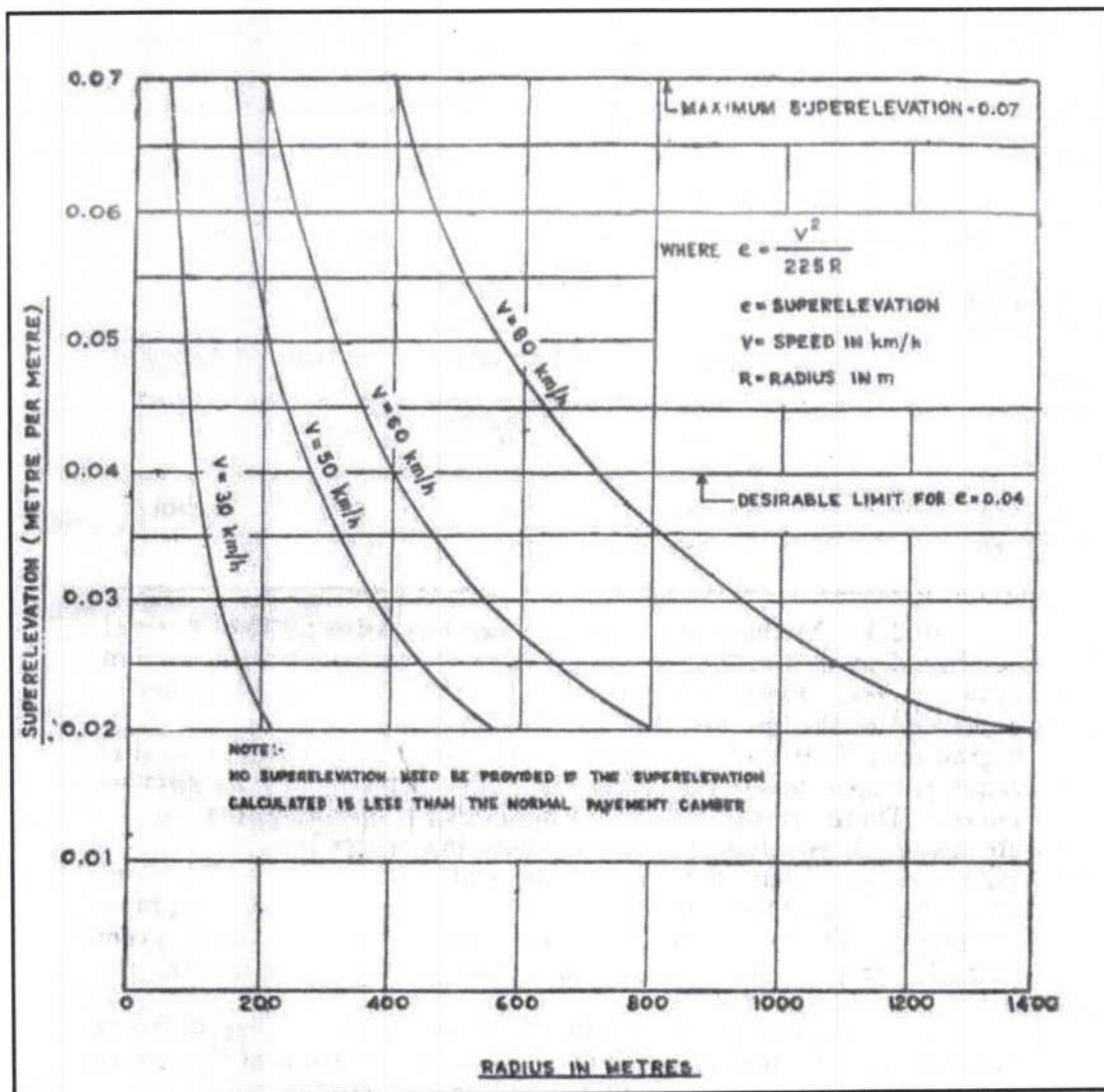
Figure 10: Values of Super Elevation
