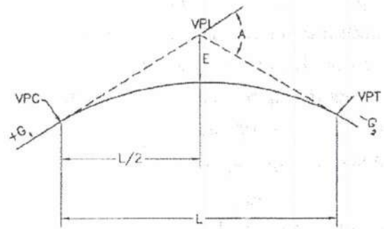
Figure 5: Summit Curve
