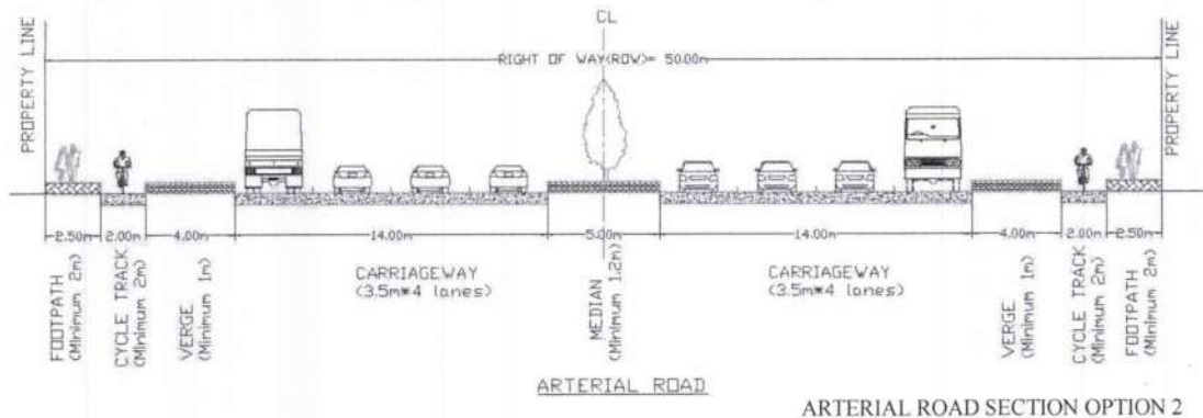
Figure 1: Typical Arterial Road Sections
