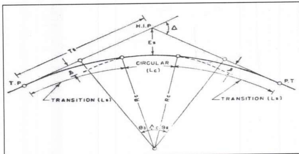
Figure 13: Elements of combined Circular and Transition Curve
