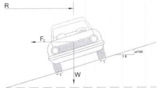
Figure 9: Supper Elevation
