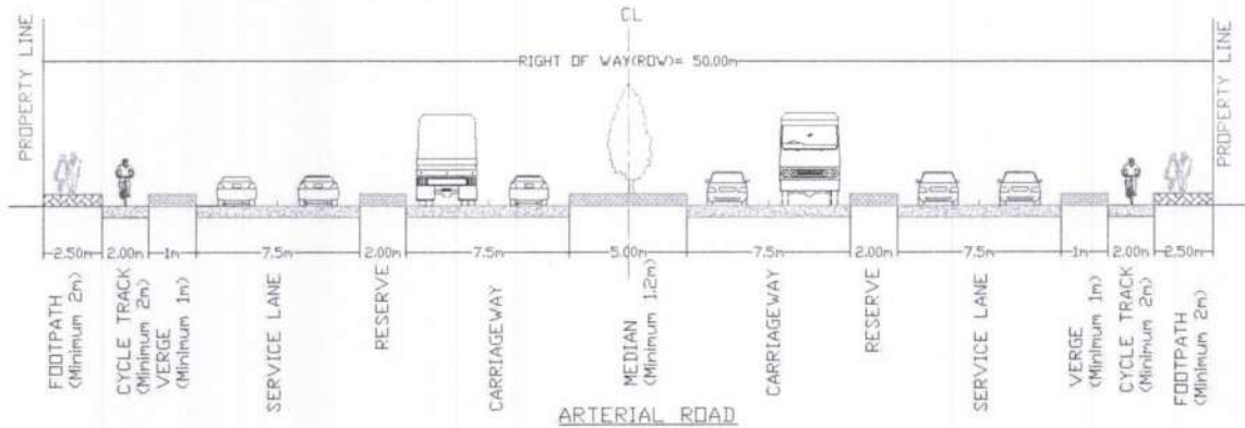
Figure 1: Typical Arterial Road Sections
